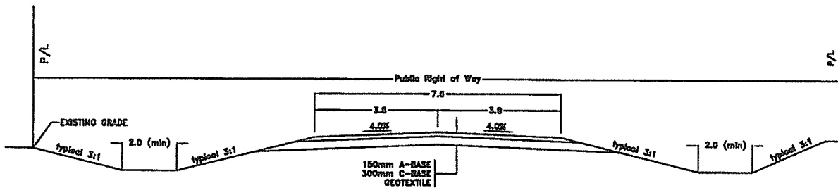
TYPICAL PUBLIC ROADWAY BASE DETAIL — GEOTEXTILE N.T.S.
